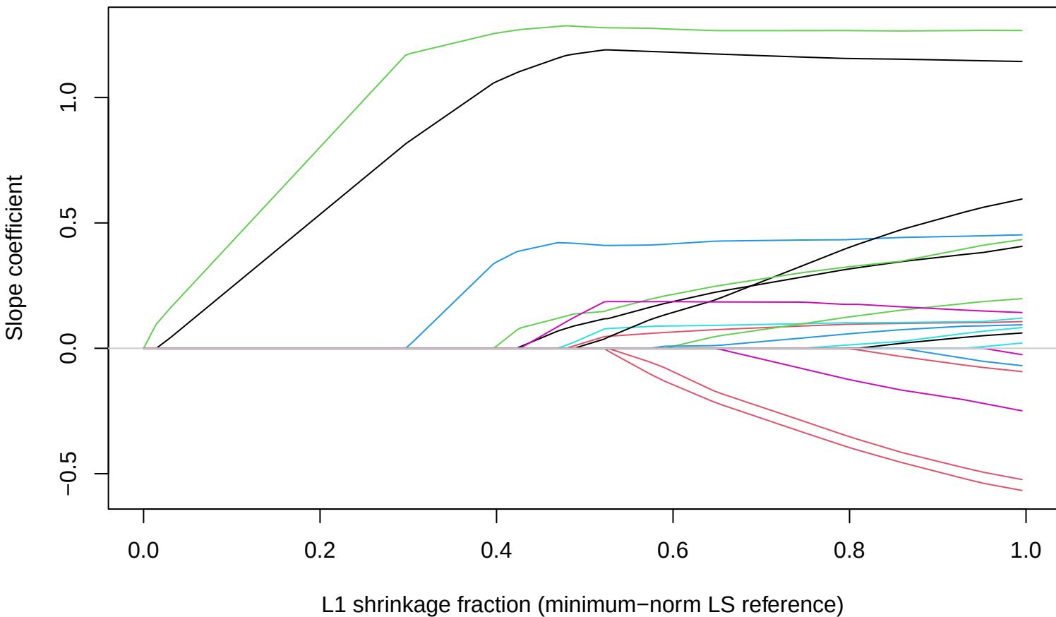
lasso coefficient path: p = 20
